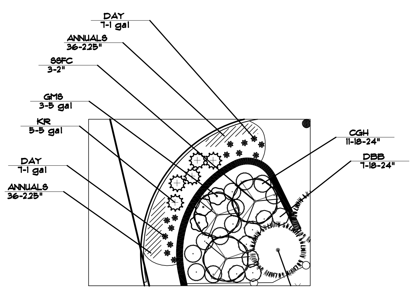
L-1.01: ENTRY PLANTING: (2 total) Scale: 1" = 10'
